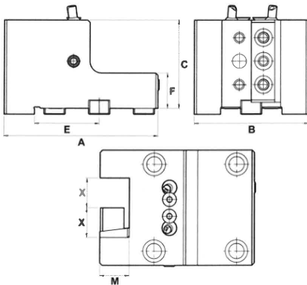
Figure L30000366: BMT Turning Holder DW700-C32-75
