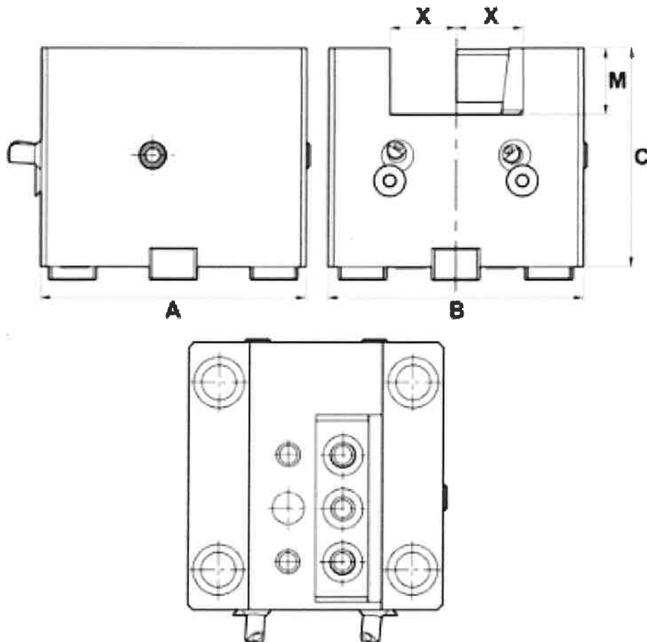
Figure L30000367. BMT Facing Holder DW700-F32-107
