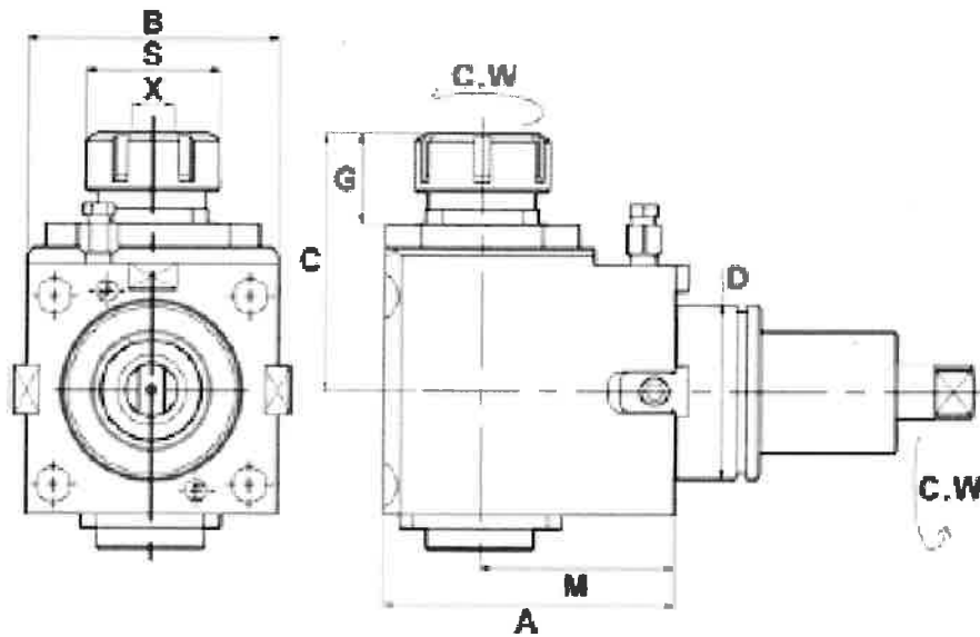
Figure L30000309: BMT Radial Drilling-Milling Head DW700-DF85-ER50-110
